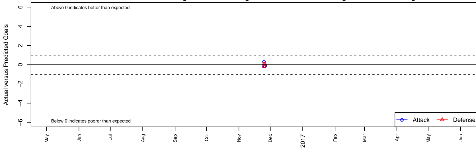
San Jose Earthquakes CV Gold B98 Dots are actual minus expected GF (blue circles) and GA (red triangles). Blue line is smoothed change in attack strength. Red is smoothed change in defense strength.
